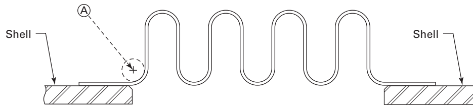
(a) U-Shaped Bellows
