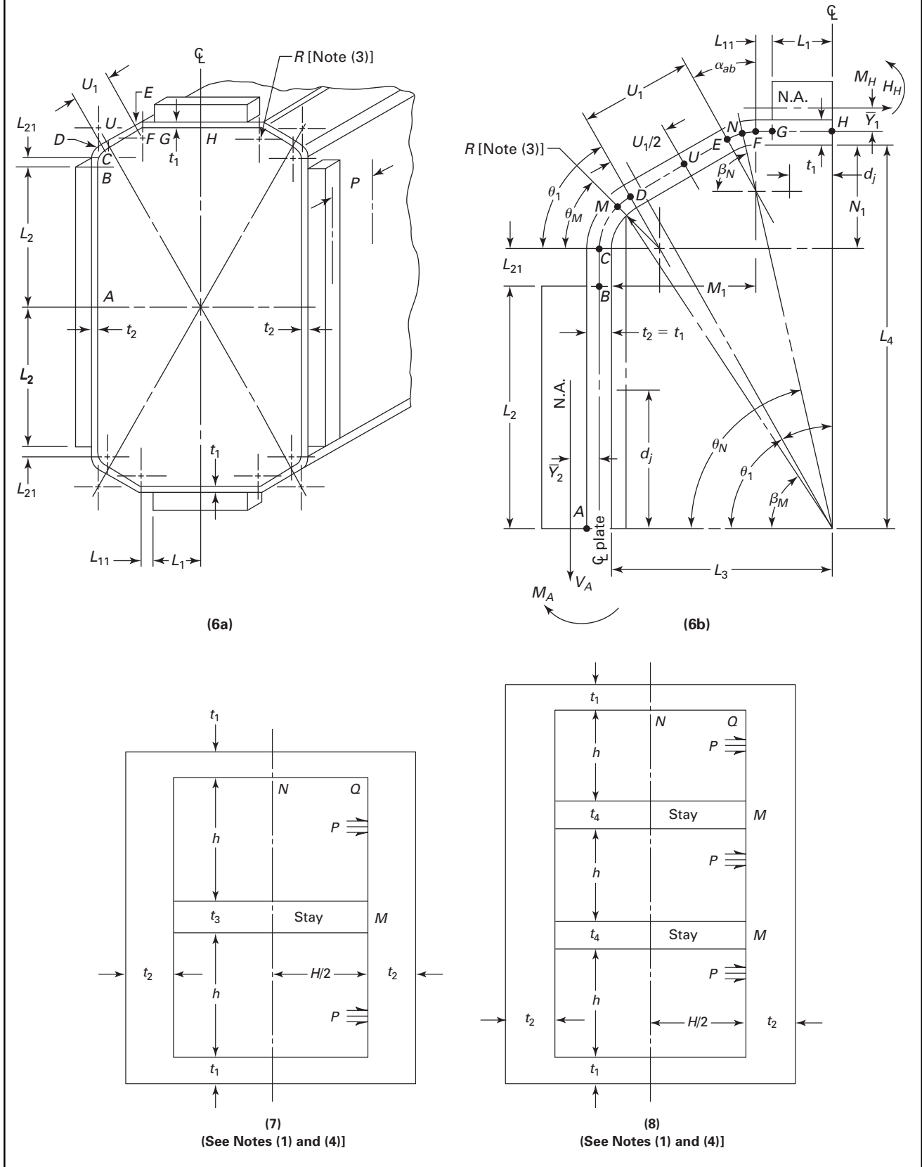
Figure 13-2(a) Vessels of Rectangular Cross Section (Cont'd)
