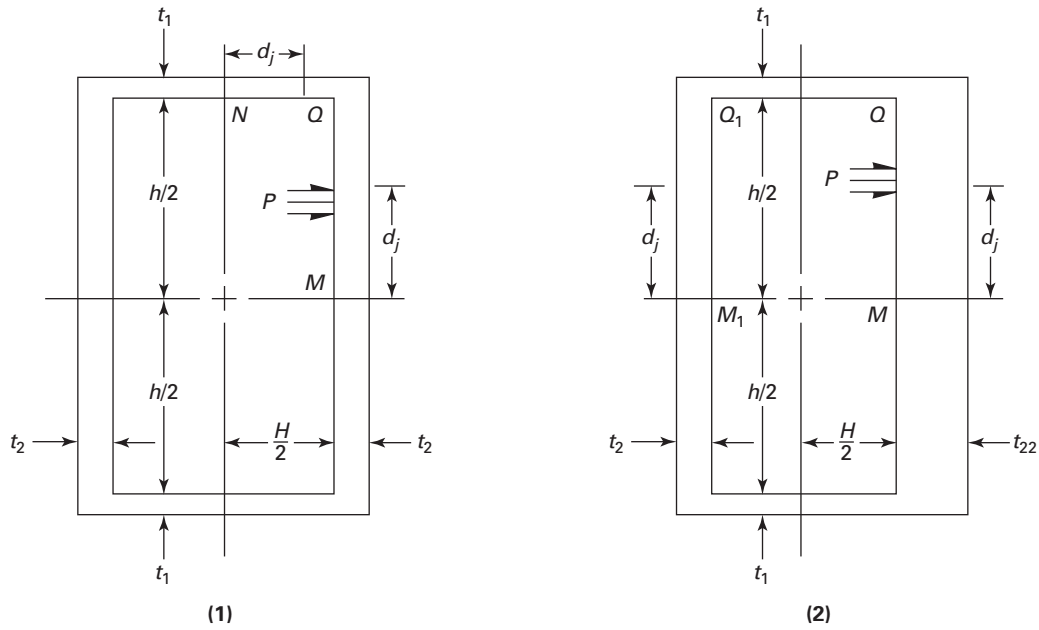
Figure 13-2(a) Vessels of Rectangular Cross Section
