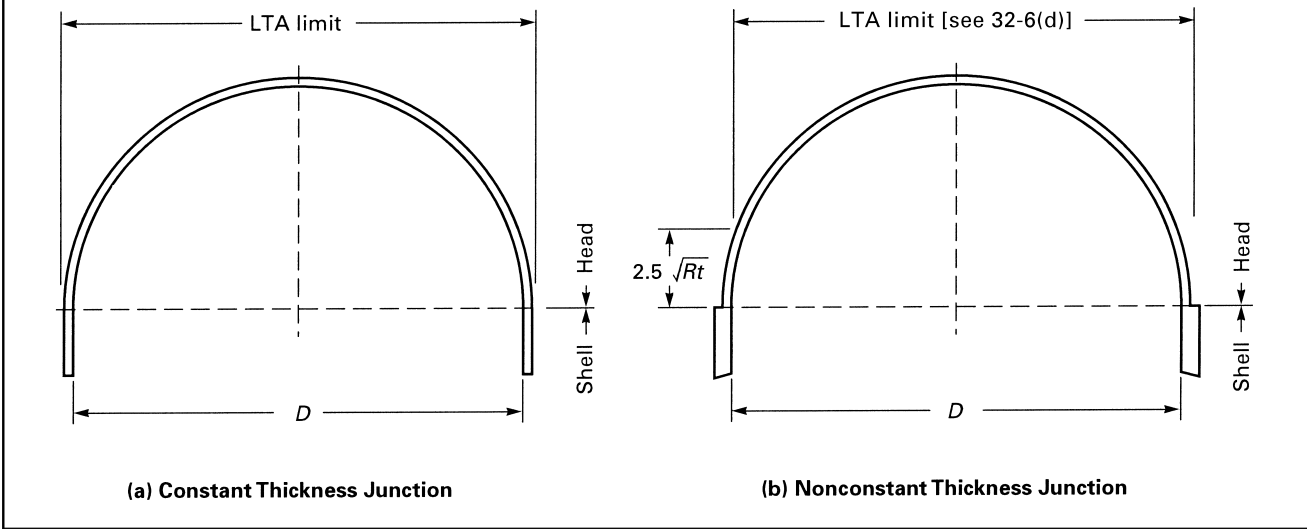
Figure 32-6.3 Limits for Hemispherical Head
