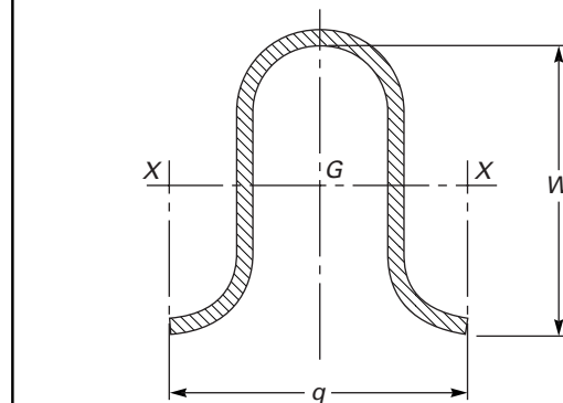
Figure 26-2 Dimensions to Determine I_{xx}
