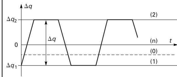
Figure 26-12 Cyclic Displacements
