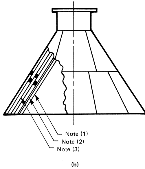
Figure ULW-2.2 Some Acceptable Layered Head Types
