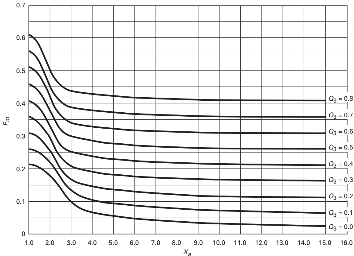
Figure UHX-13.3-1 F_m Versus X_a ( 0.0 \leq Q_3 \leq 0.8 )
