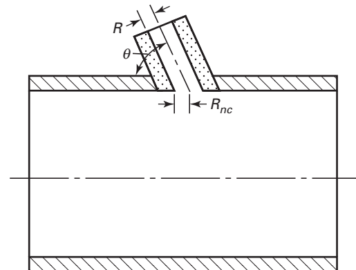
Figure 1-10-4 Nozzle in a Cylindrical Shell Oriented at an Angle From the Longitudinal Axis
