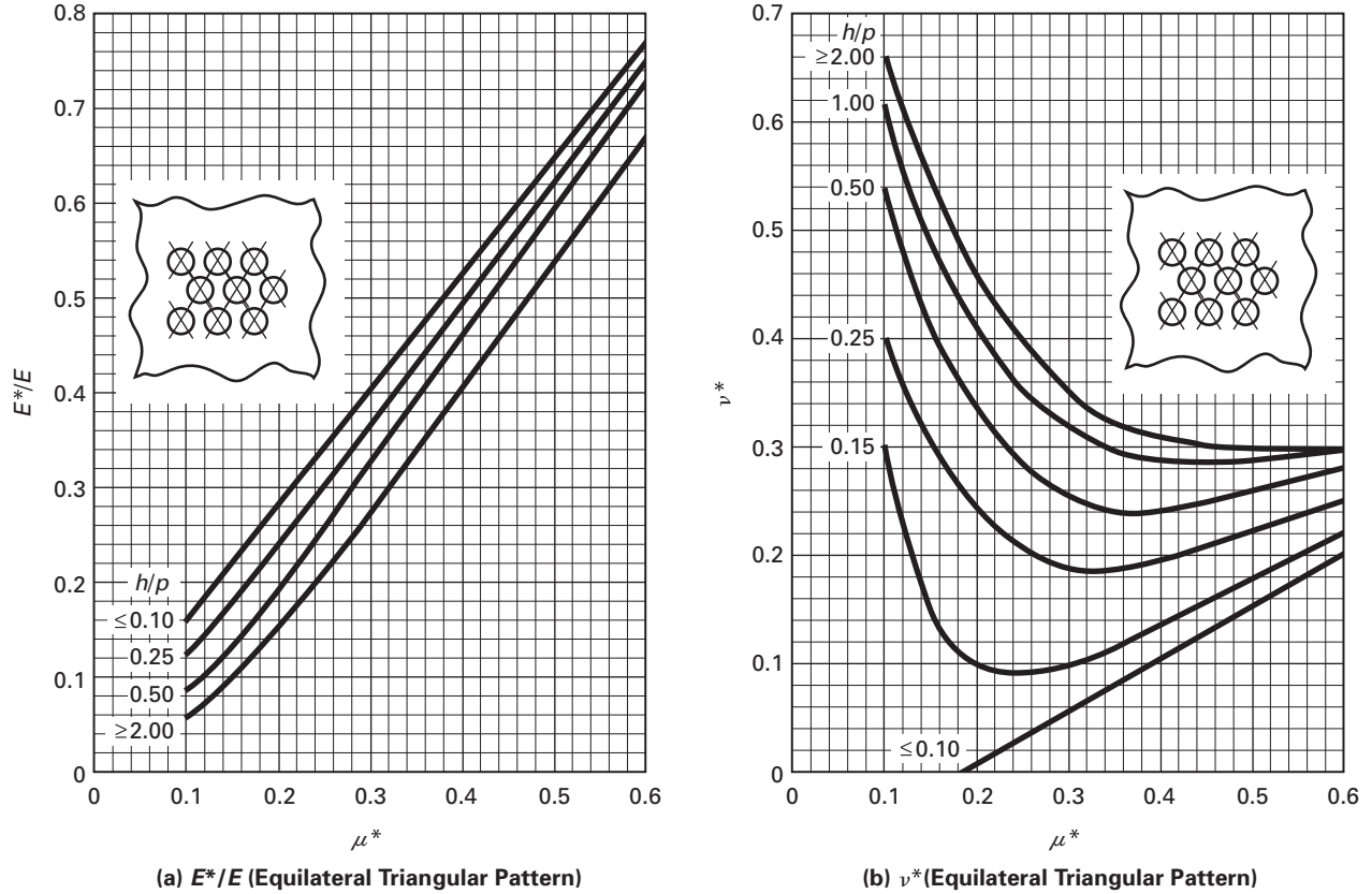
(a) Equilateral Triangular Pattern: E^*/E = \alpha_0 + \alpha_1\mu^* + \alpha_2\mu^{*2} + \alpha_3\mu^{*3} + \alpha_4\mu^{*4}
