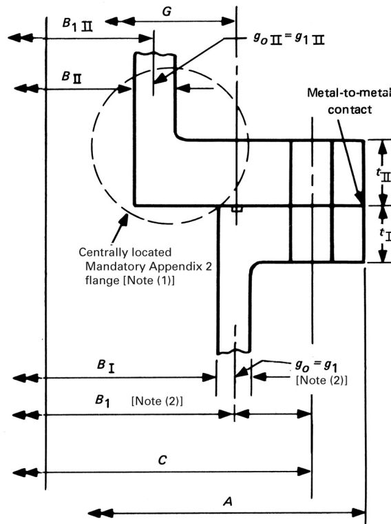
Figure Y-5.1.2 Class 2 Flange Assembly
