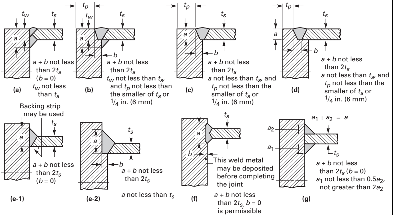
Typical Unstayed Flat Heads, Tubesheets Without a Bolting Flange, and Side Plates of Rectangular Vessels [See Note (1)]
