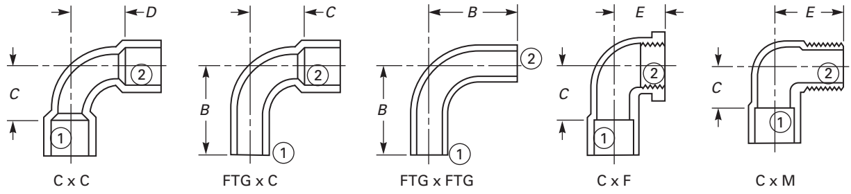
Fig. 1 Method of Designating Laying Lengths of Fittings and Openings of Reducing Fittings (Cont'd)
