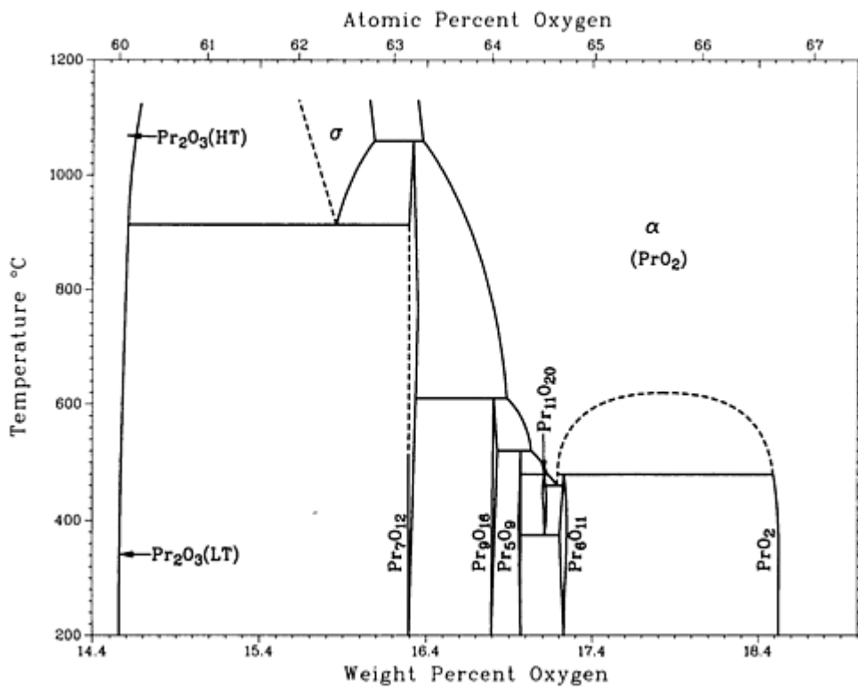
O-Pr phase diagram
