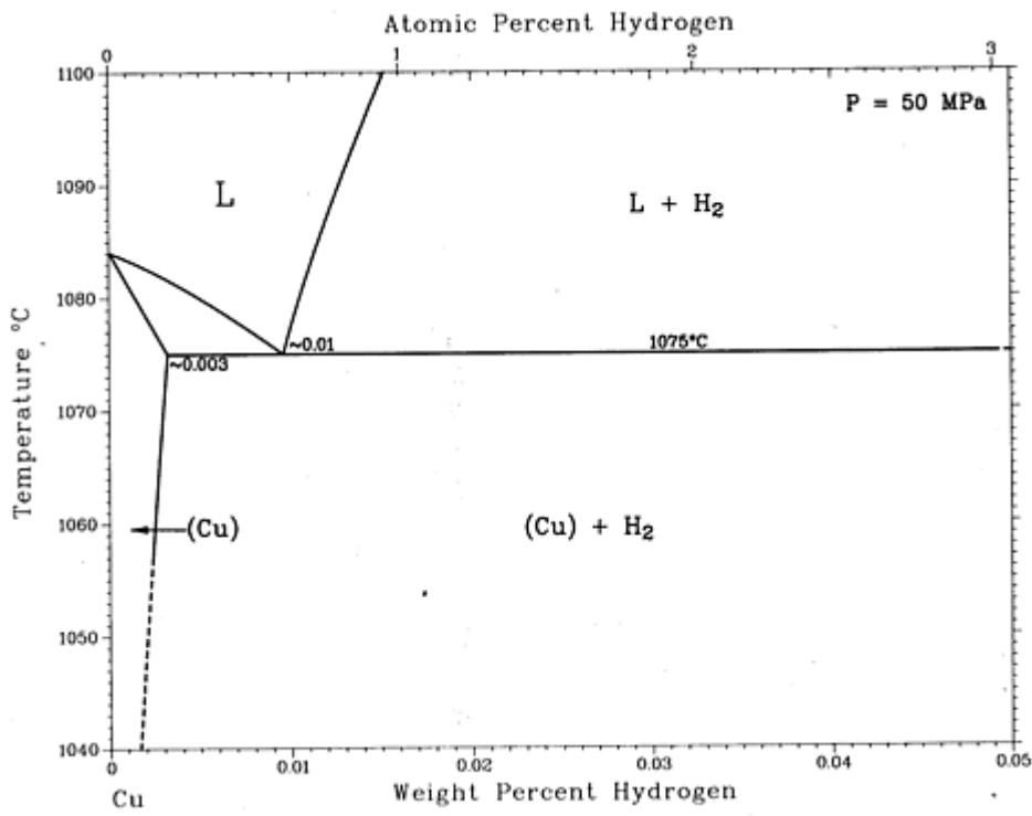
Cu-H phase diagram
