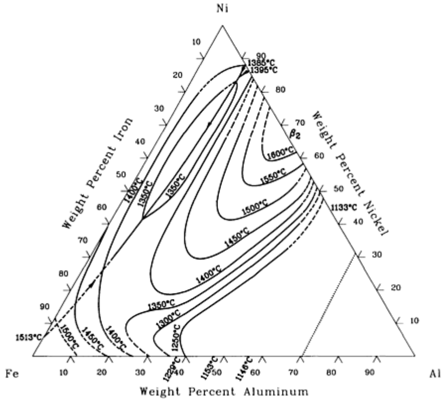
Al-Fe-Ni liquidus projection [88Ray 60].
