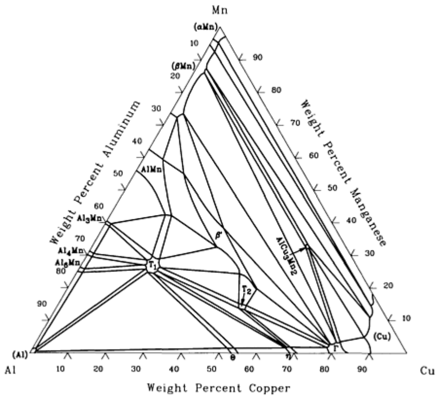
Al-Cu-Mn isothermal section at 25 °C [66Kos 21].
