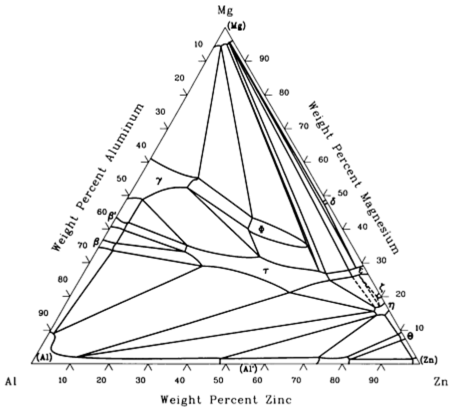
Al-Mg-Zn isothermal section at 335 °C [73Wil 34].
