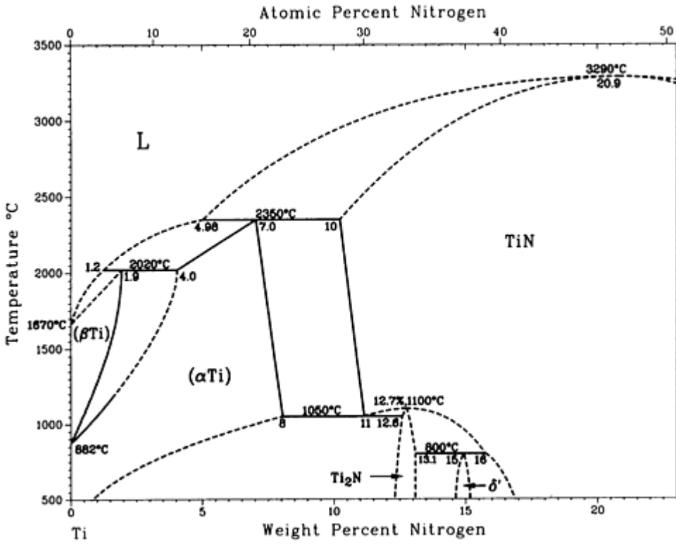
N-Ti phase diagram
