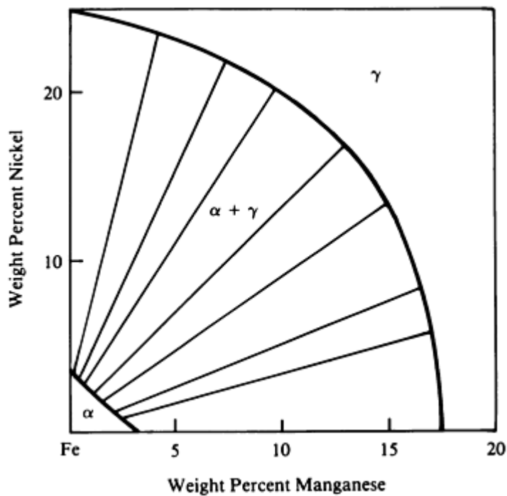
Fe-Mn-Ni isothermal section at 550 °C [89Har 63].
