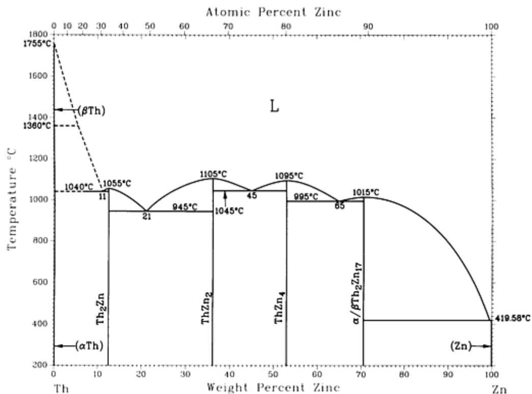
Th-Zn phase diagram
