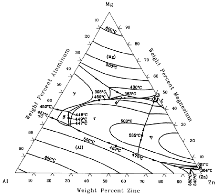
Al-Mg-Zn liquidus projection [73Wil 34].
