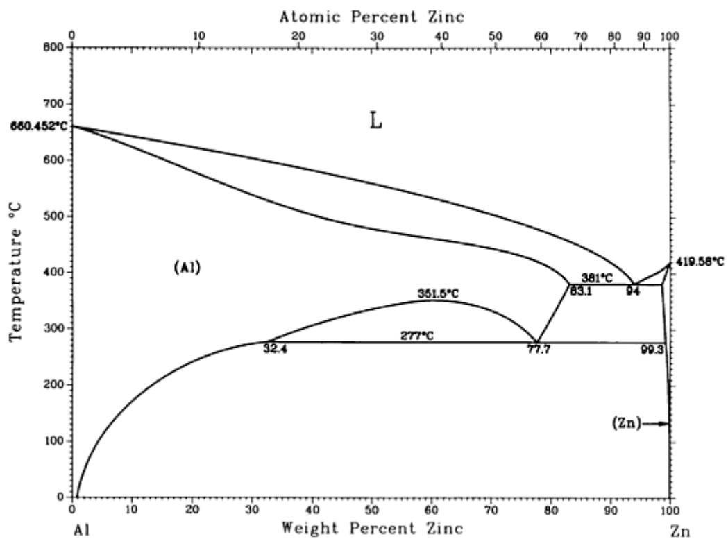
Al-Zn phase diagram
