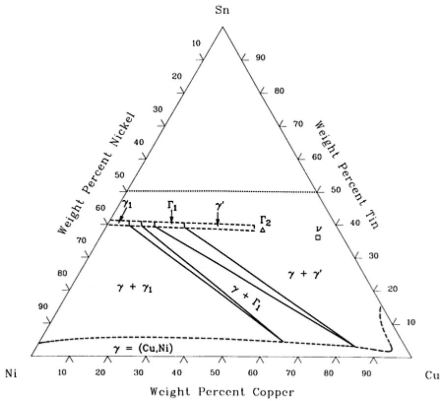
Cu-Ni-Sn isothermal section at 550 °C [90Gup 64].
