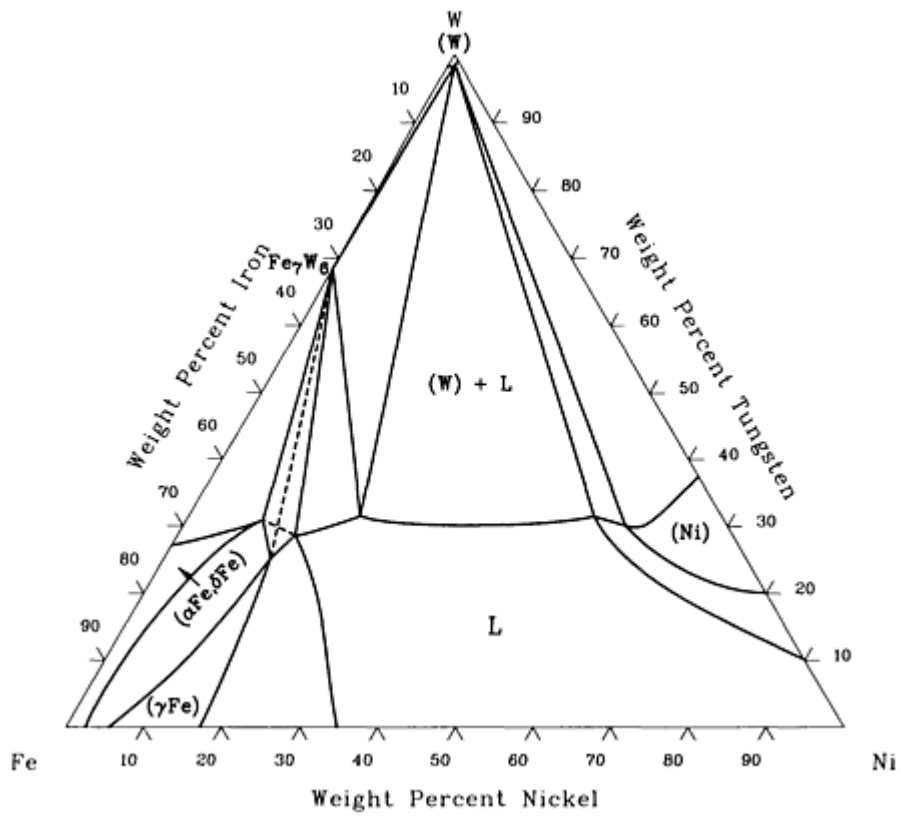
Fe-Ni-W isothermal section at 1465 °C [88Ray 60].
