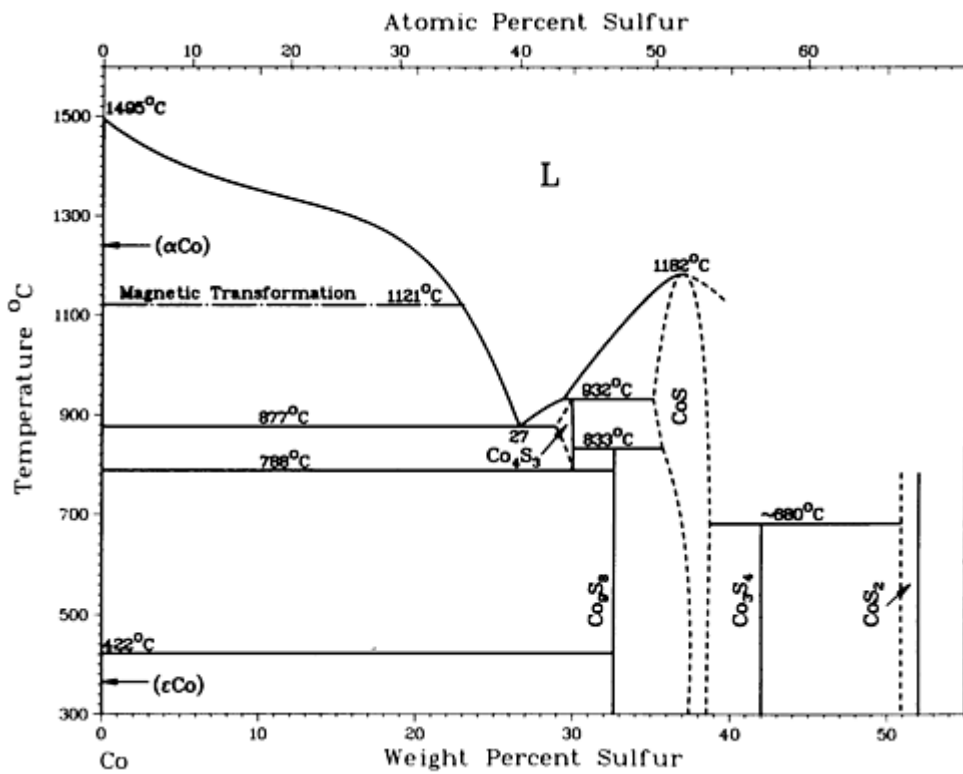
Co-S phase diagram
