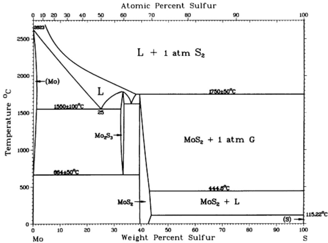
Mo-S phase diagram
