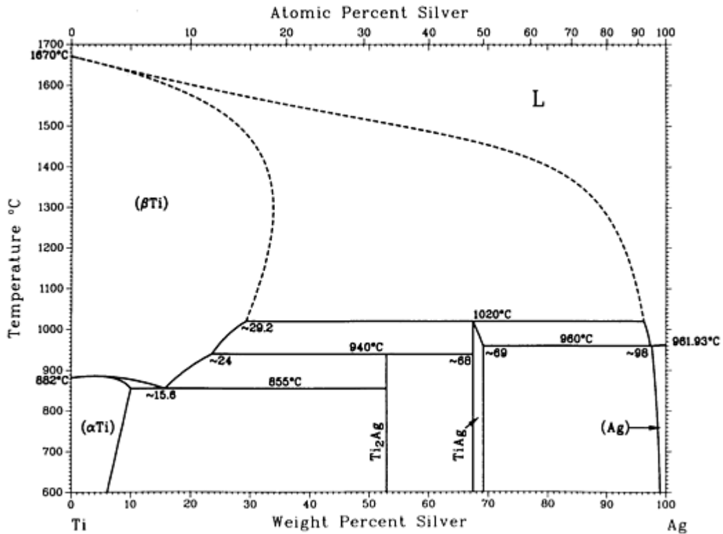
Ag-Ti phase diagram
