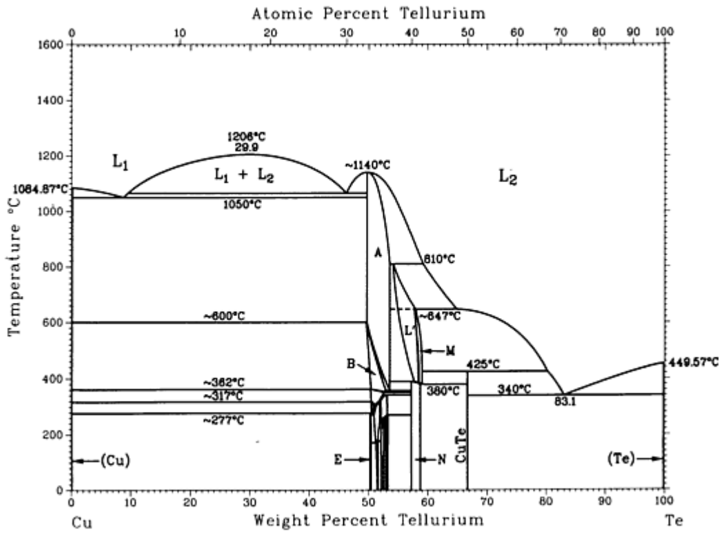
Cu-Te phase diagram
