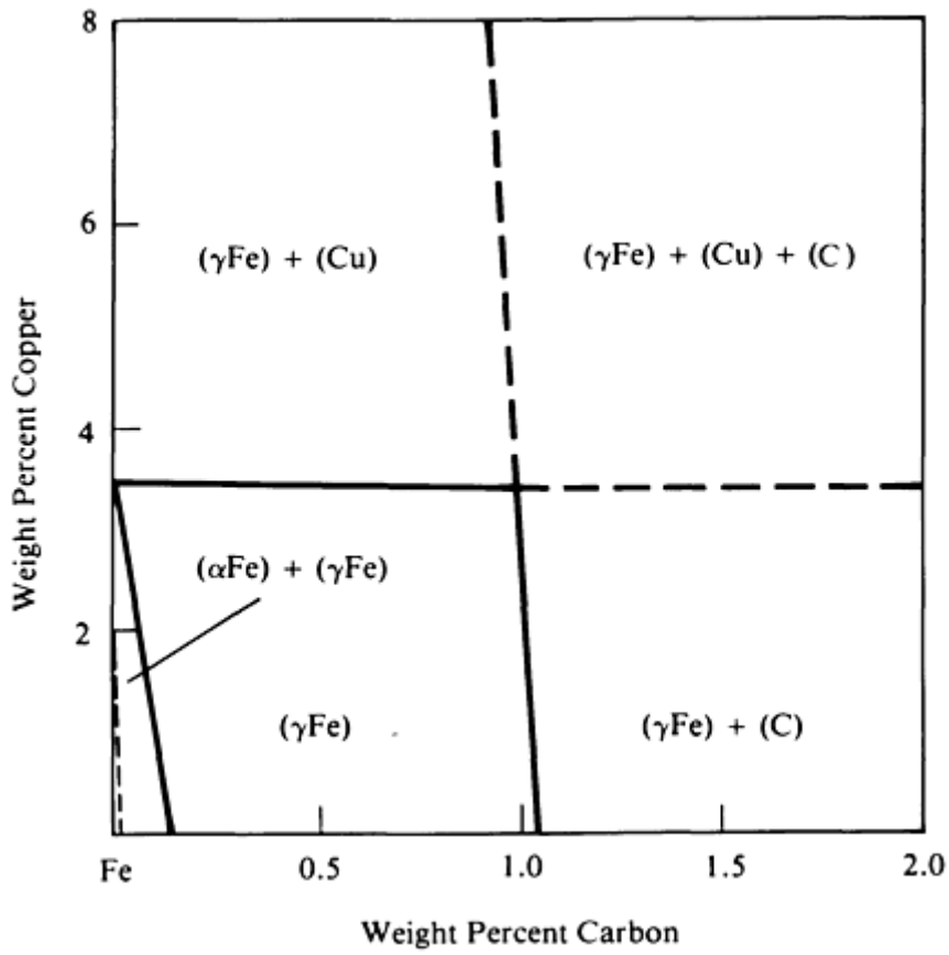
C-Cu-Fe isothermal section at 850 °C [88Ray 60].
