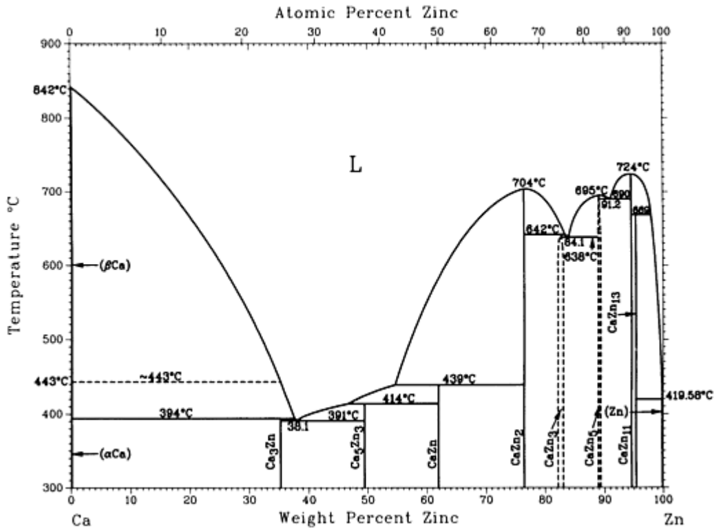
Ca-Zn phase diagram
