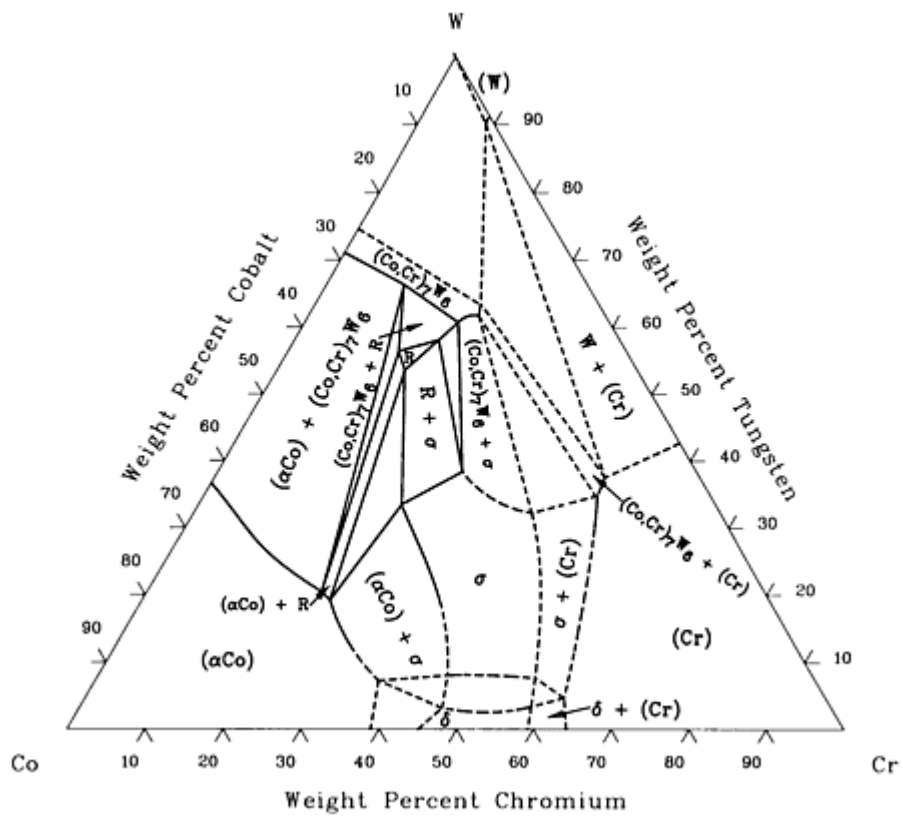
Co-Cr-W isothermal section at 1350 °C [73Dra 29].
