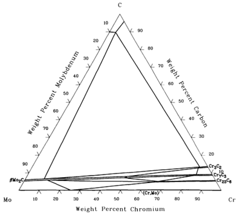
C-Cr-Mo isothermal section at 1350 °C [65Kuz 19].
