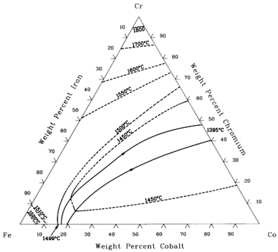
Co-Cr-Fe solidus projection [88Ray 60].
