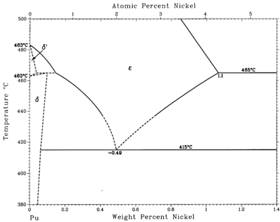
Pu-rich region of the Pu-Ni phase diagram
