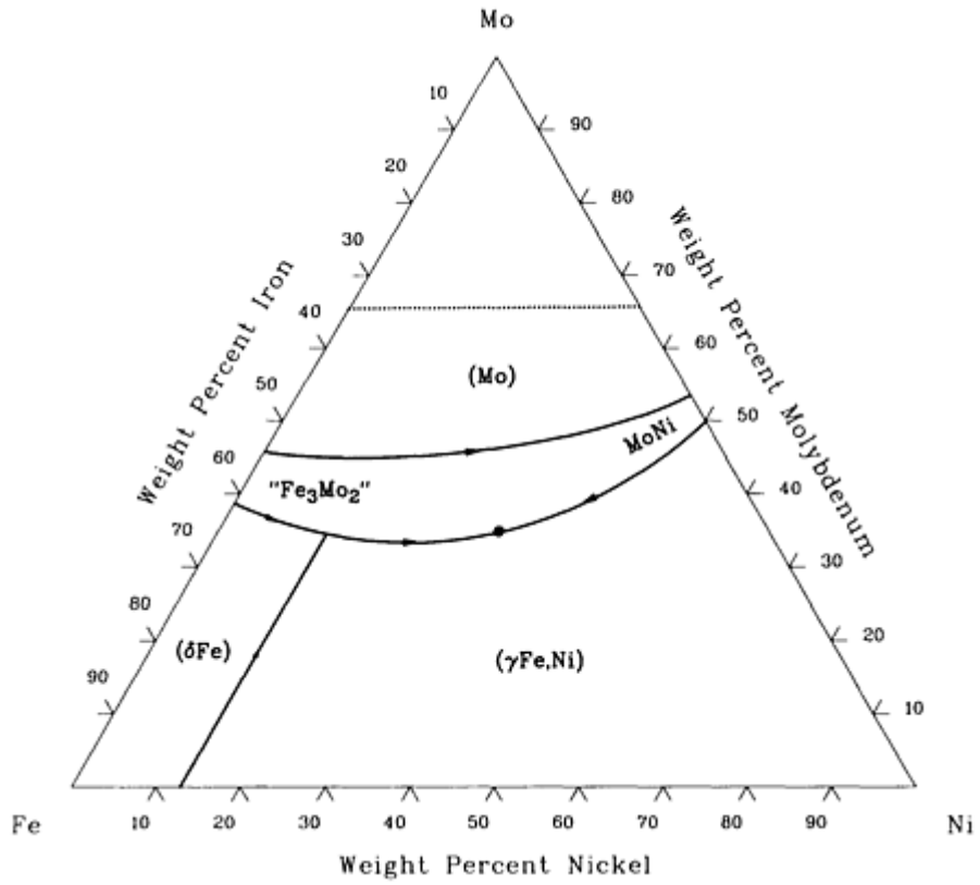
Fe-Mo-Ni liquidus projection [36Kos 3].
