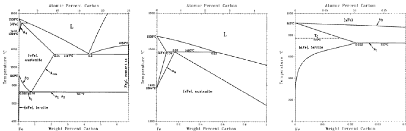
Fig. 45 The iron-cementite phase diagram and details of the ( \delta Fe) and ( \alpha Fe) phase fields. Source: Adapted
